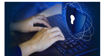
Endpoint Security
